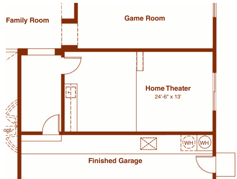
OPTIONAL HOME THEATER I.L.O. GARAGE
