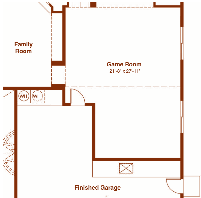
OPTIONAL EXTENDED GAME ROOM I.L.O. GARAGE
